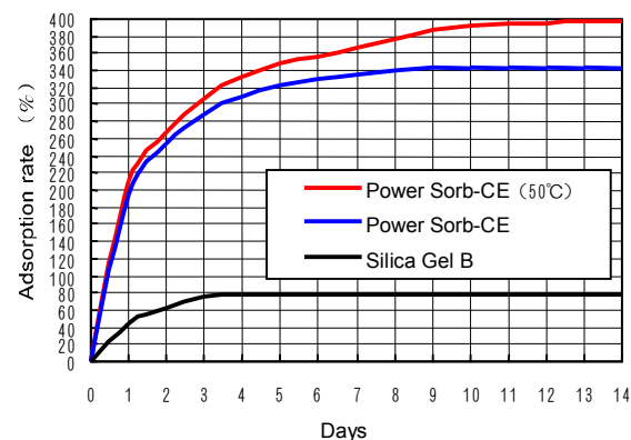
Fig. 2 Adsorption rate (25°C, RH90%)
